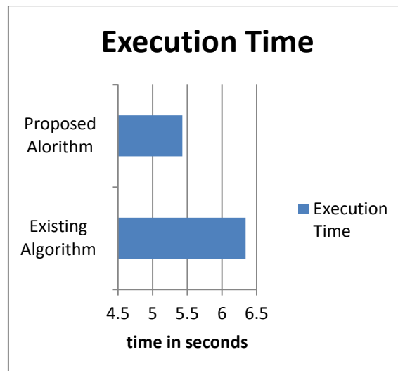
Fig 2: Execution time
