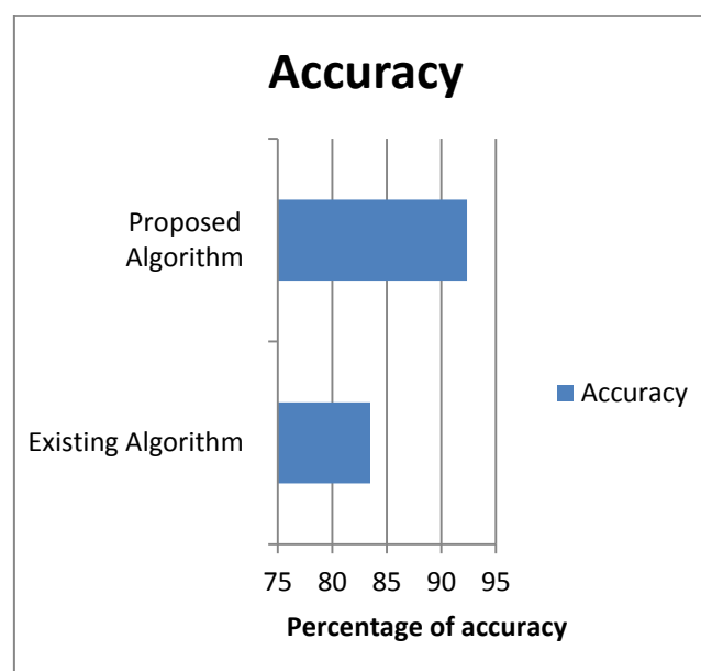
Fig 1: Accuracy Comparison
