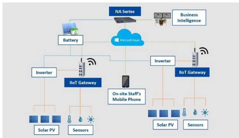
Fig 2: Energy Management System in the Smart grid Infrastructure
