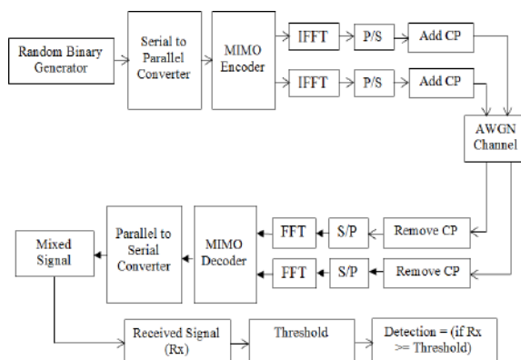
Figure 4: Design of MIMO-OFDM System using Matched Filter Spectrum Sensing Cognitive Radio Network
