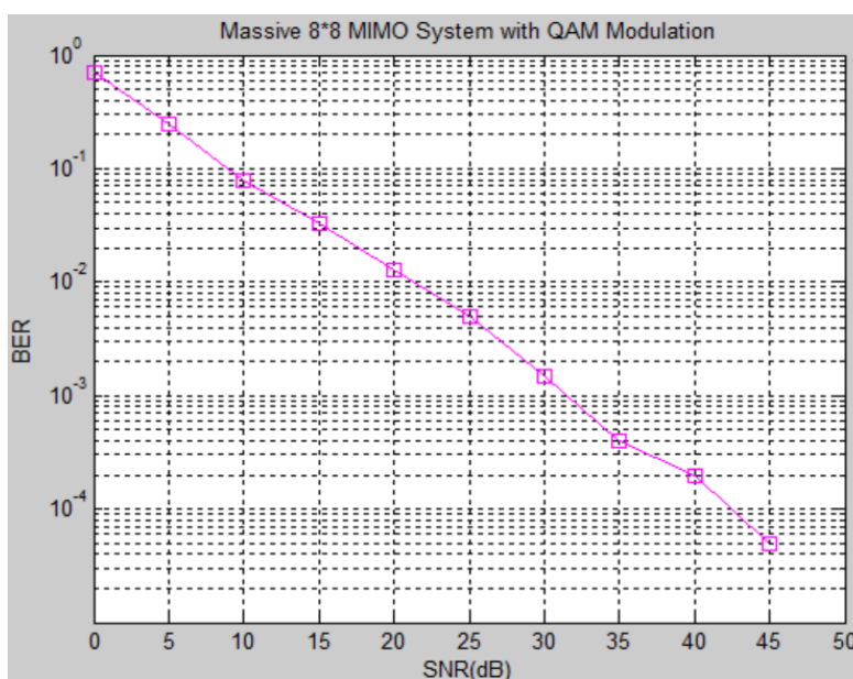
Figure 5: BER vs SNR for Matched Filter Detection Spectrum Sensing 8 \times 8 System
