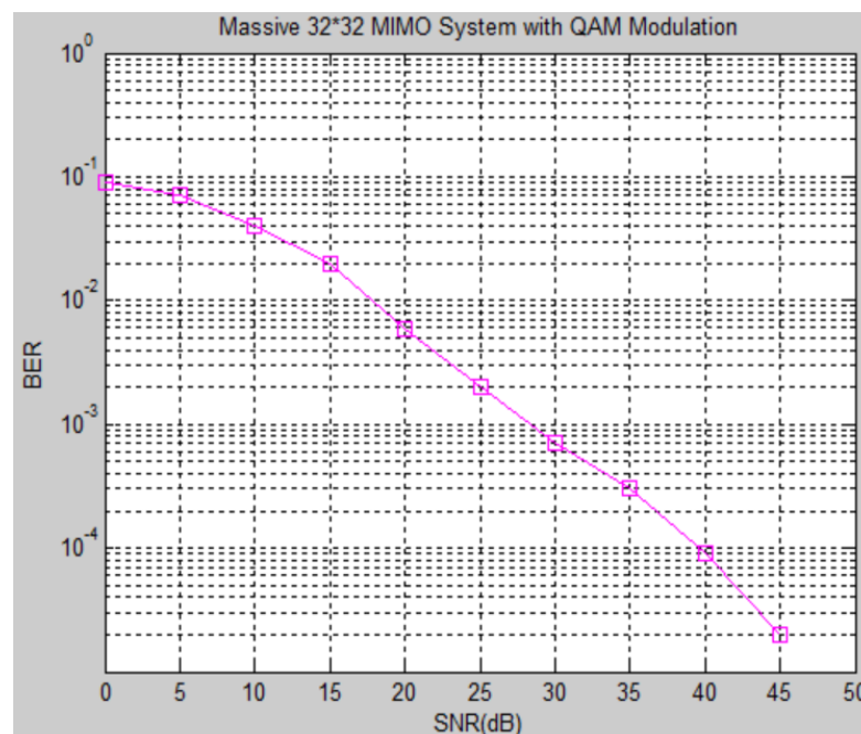
Figure 7: BER vs SNR for Matched Filter Detection Spectrum Sensing 32 \times 32 System
