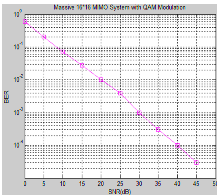
Figure 6: BER vs SNR for Matched Filter Detection Spectrum Sensing 16 \times 16 System
